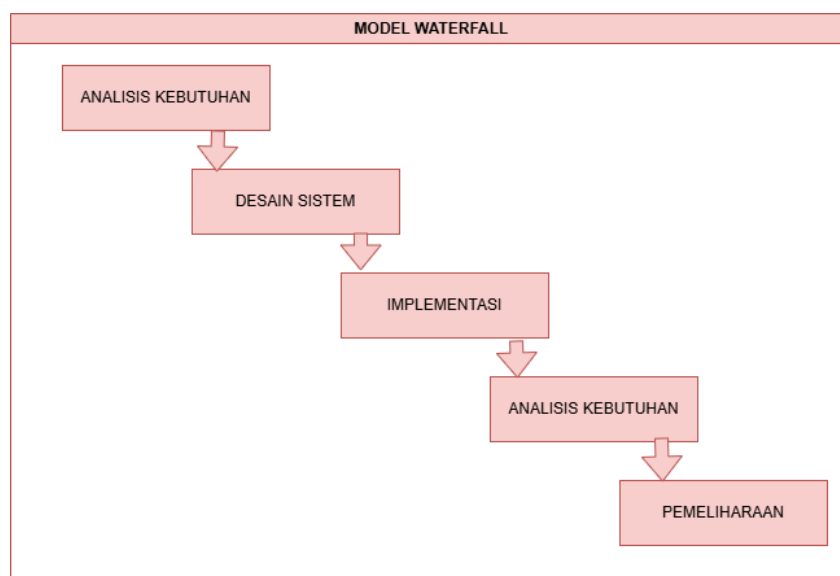
Gambar 1. Model Waterfall
